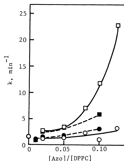
Fig. 4. Effects of azobenzene derivatives on the rates of the BTB release from DPPC liposomes at 25°C: —○—, trans- C_4 Azo; —□—, cis- C_4 Azo; —●—, trans- C_2 Azo; —■—, cis- C_2 Azo. The cis-isomers were prepared by irradiating the liposome solutions at 366-nm light for 5 min.
