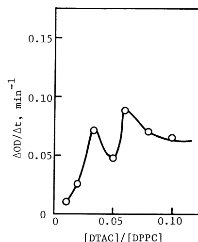
Fig. 3. Effects of DTAC on the shrinkage rates of DPPC liposomes at 25°C.
