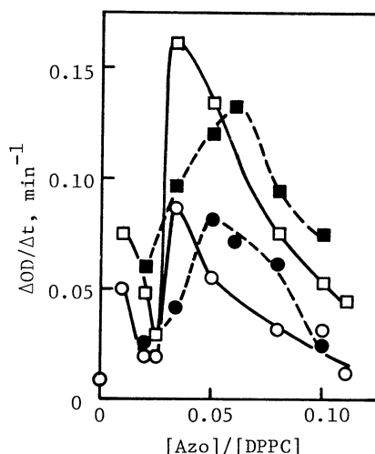
Fig. 2. Effects of the azobenzene derivatives on the shrinkage rates of the DPPC liposomes at 25°C: ○—○, trans-C 4 Azo; □—□, cis-C 4 Azo; ●—●, trans-C 2 Azo; ■—■, cis-C 2 Azo. The cis-isomers were prepared by irradiating the liposome solutions at 366-nm light for 5 min.
