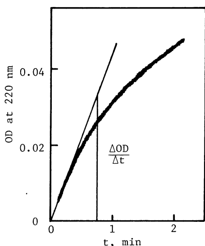
Fig. 1. Time-dependent absorption change of trans-C 4 Azo loading DPPC liposomes at 25°C: [trans-C 4 Azo]/[lipid] = 1/10. The optical density at t = 0 was chosen arbitrarily.
